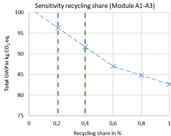
Fig. 6-1: Total GWP of the window manufacturing module (A1–A3) depending on the recycle content
